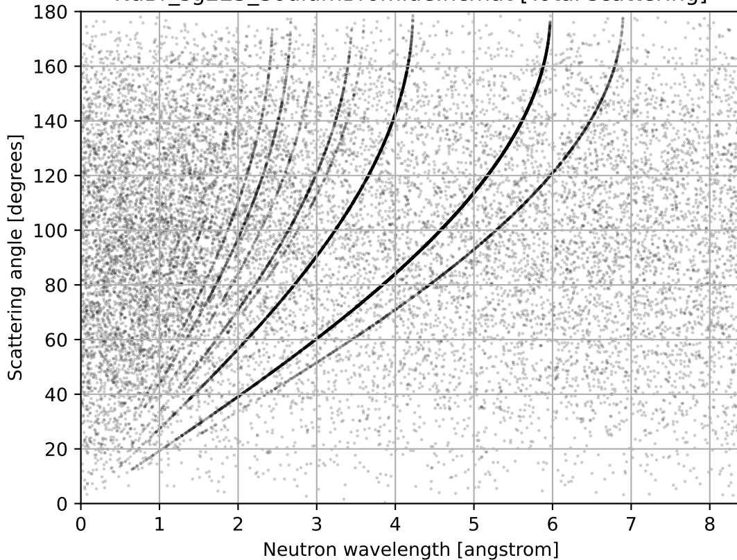
NaBr_sg225_SodiumBromide.ncmat [Total scattering]
