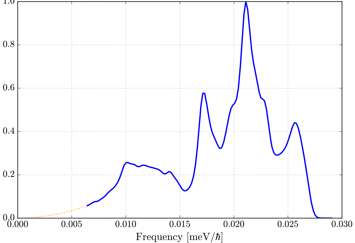
Phonon DOS (VDOS) for Na in NaCl_sg225_SodiumChloride.ncmat
