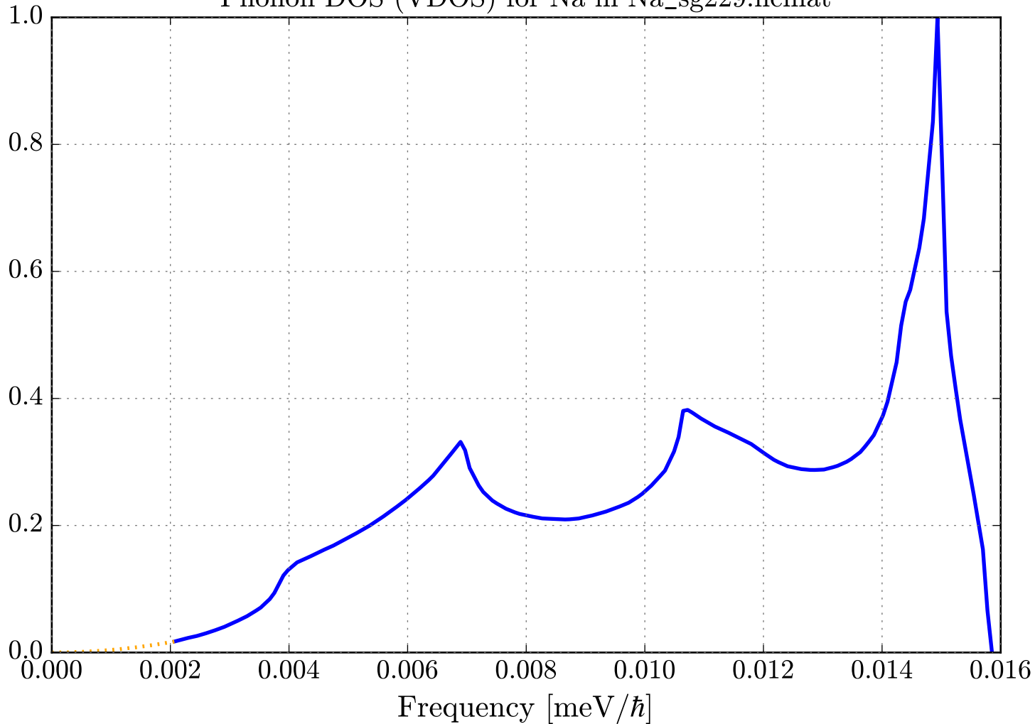
Phonon DOS (VDOS) for Na in Na_sg229.ncmat
