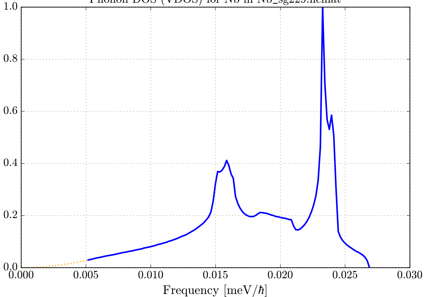
Phonon DOS (VDOS) for Nb in Nb_sg229.ncmat
