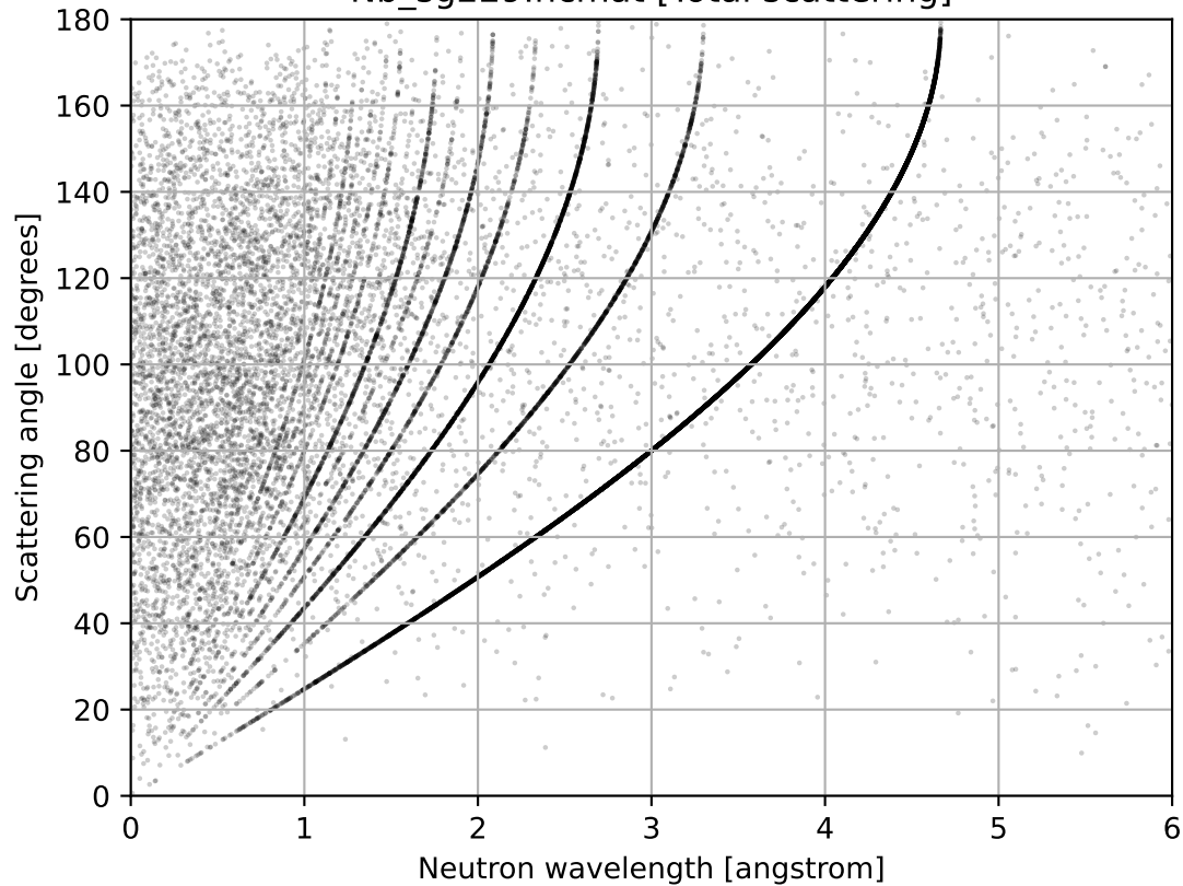
Nb_sg229.ncmat [Total scattering]
