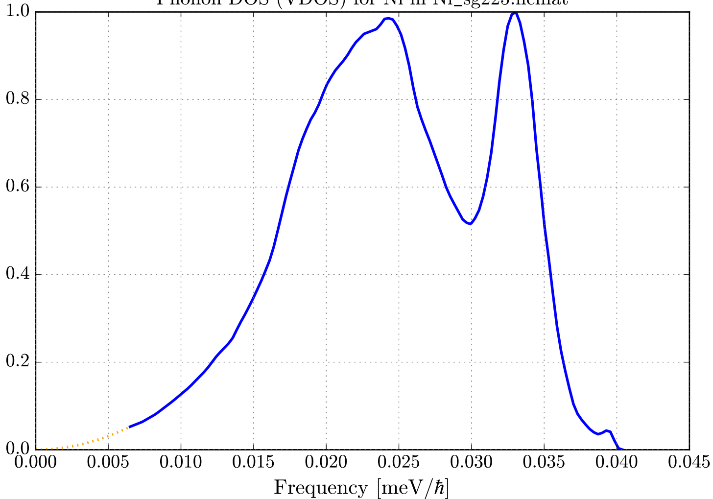
Phonon DOS (VDOS) for Ni in Ni_sg225.ncmat
