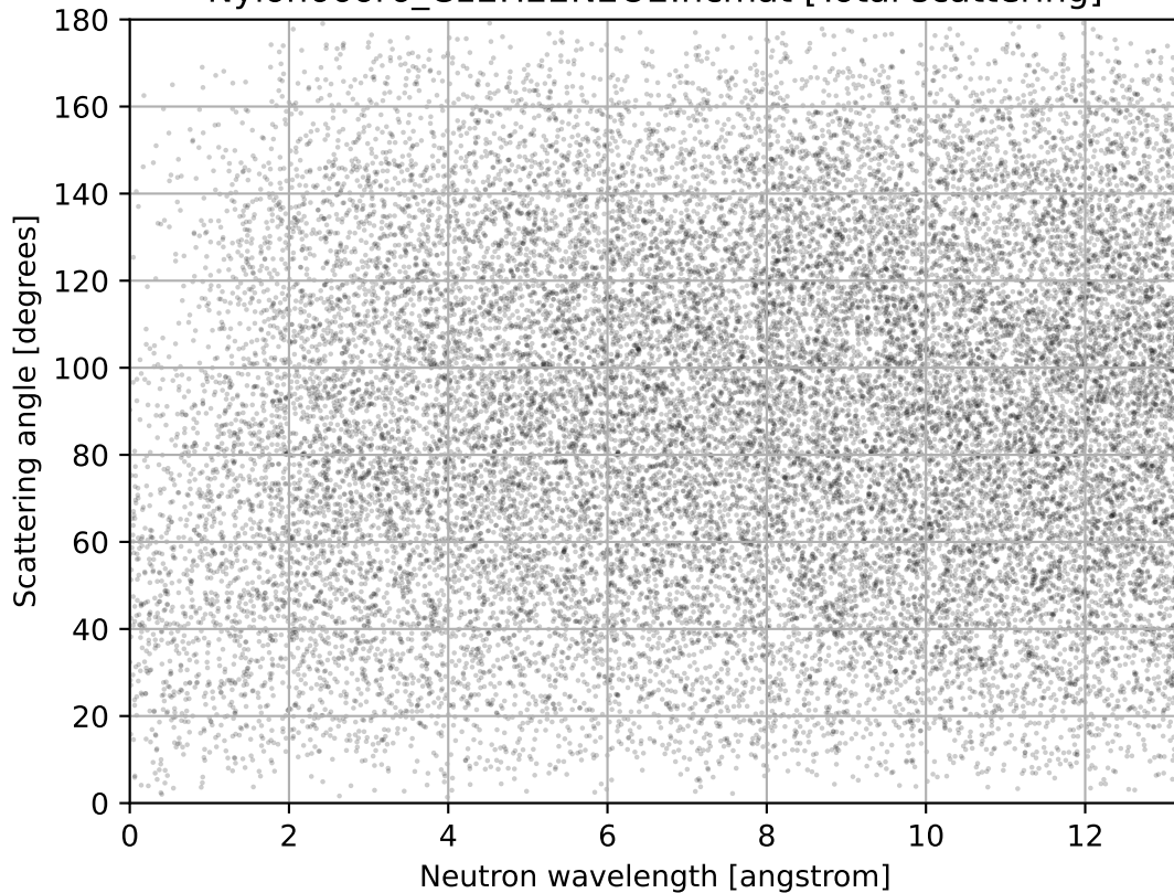
Nylon66or6_C12H22N2O2.ncmat [Total scattering]
