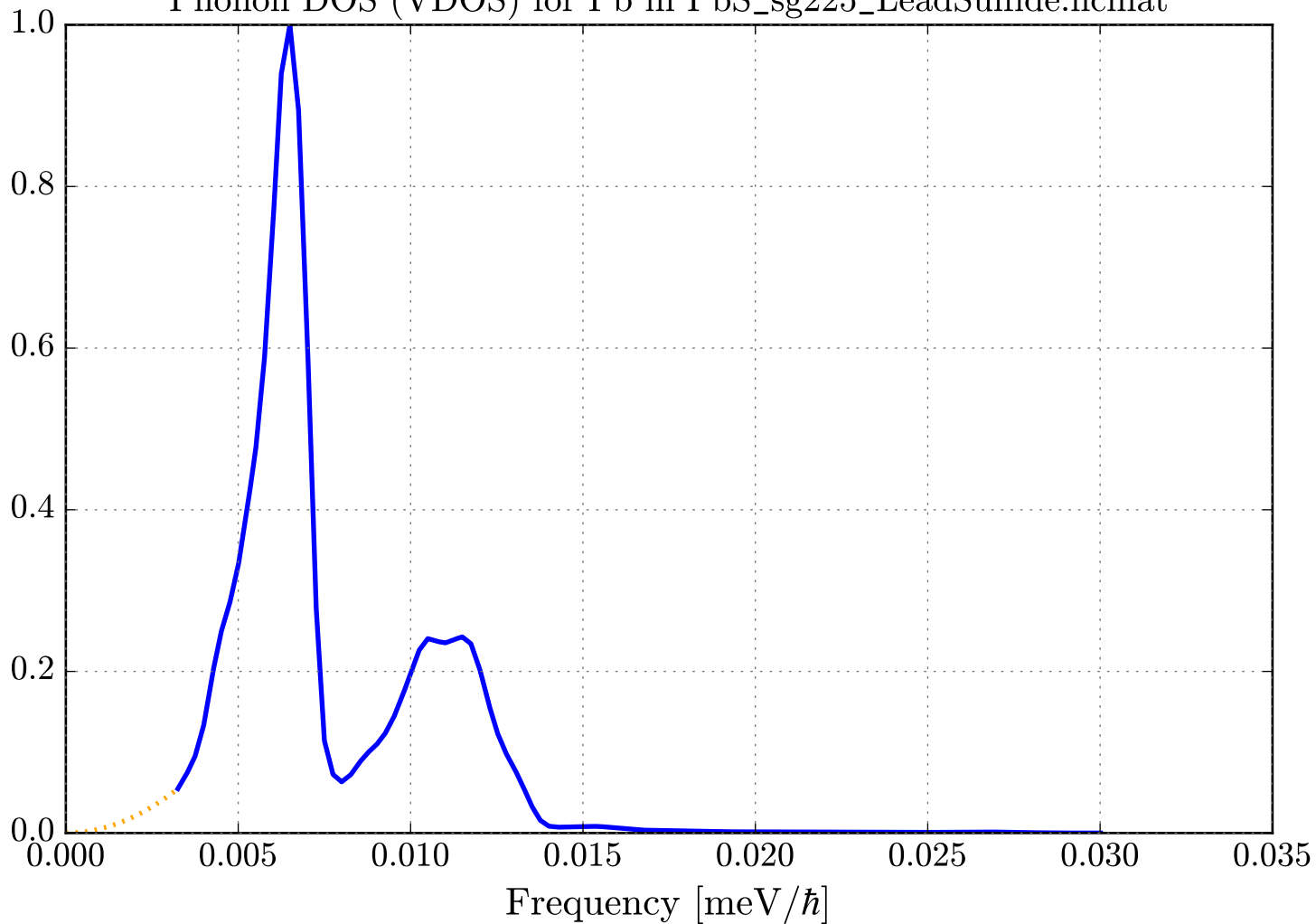
Phonon DOS (VDOS) for Pb in PbS_sg225_LeadSulfide.ncmat
