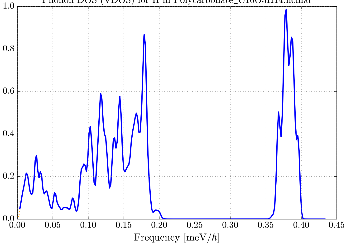
Phonon DOS (VDOS) for H in Polycarbonate_C16O3H14.ncmat
