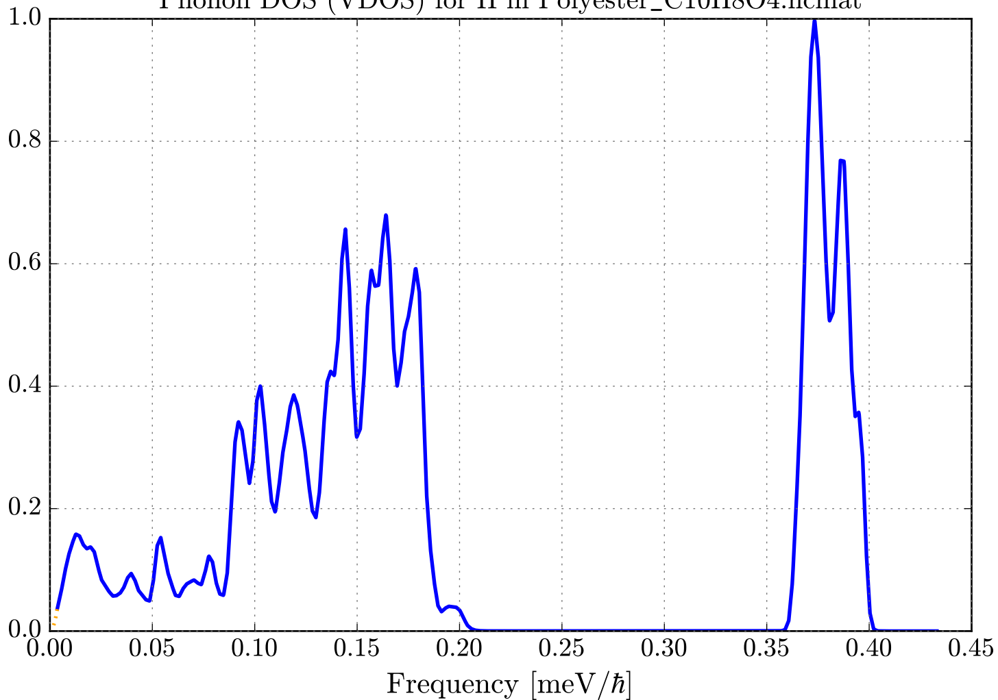
Phonon DOS (VDOS) for H in Polyester_C10H8O4.ncmat
