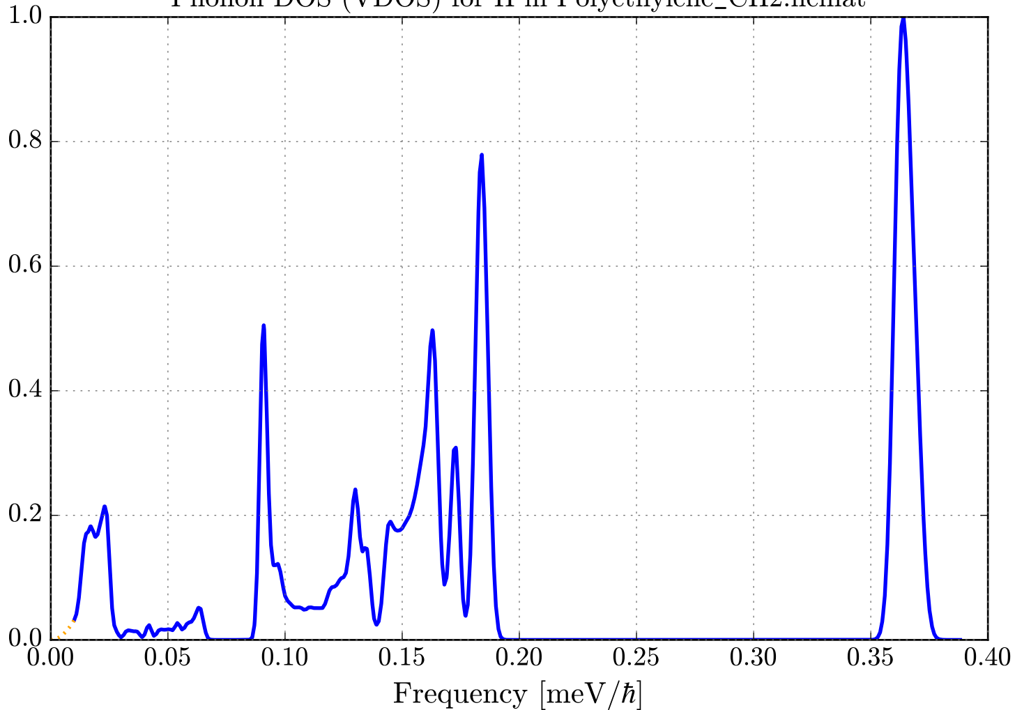
Phonon DOS (VDOS) for H in Polyethylene_CH2.ncmat
