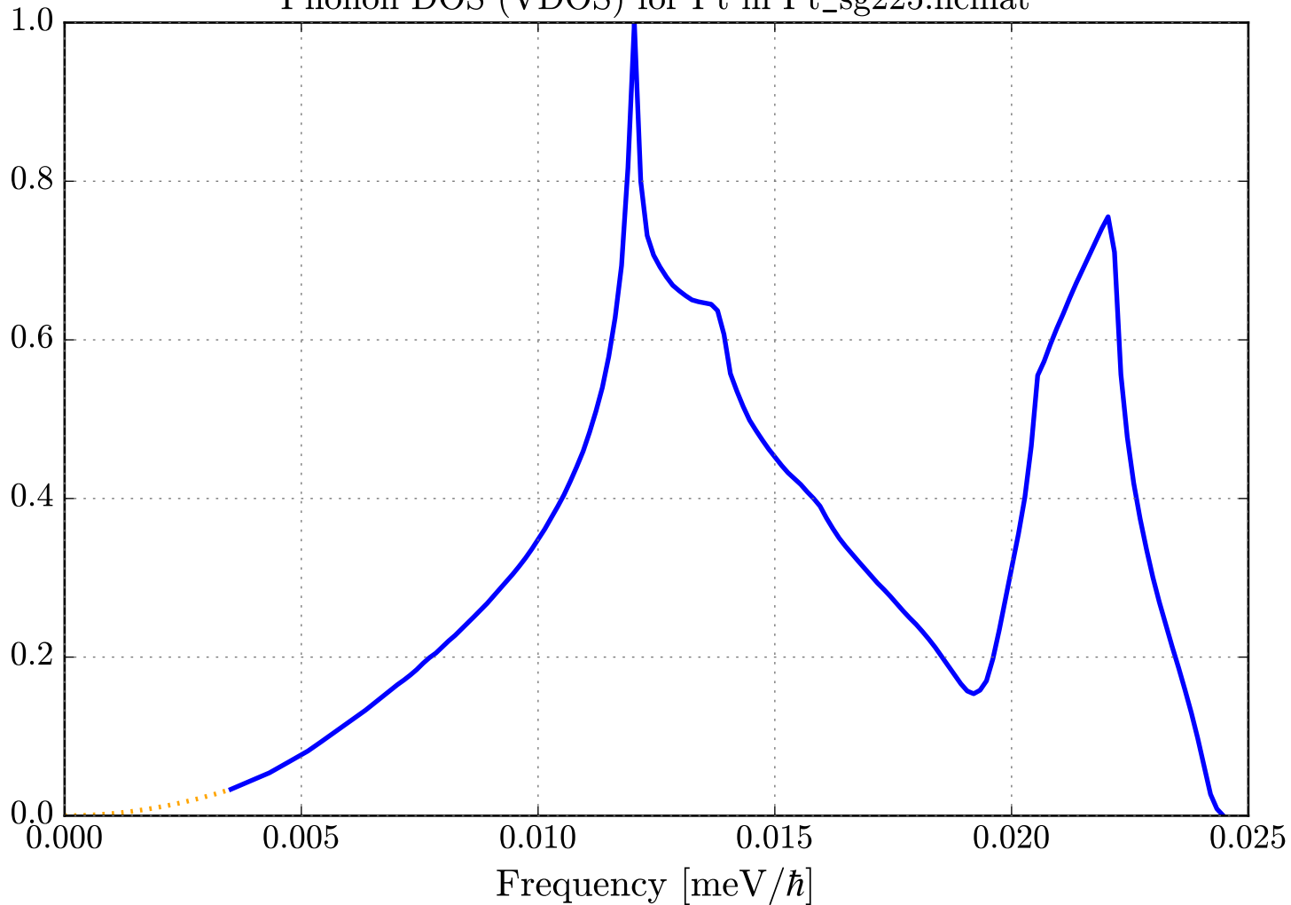
Phonon DOS (VDOS) for Pt in Pt_sg225.ncmat
