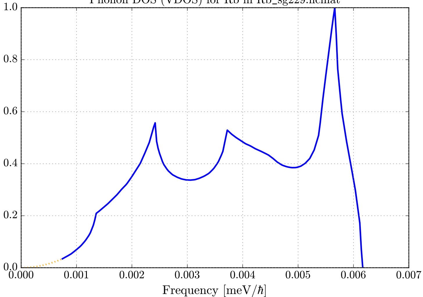
Phonon DOS (VDOS) for Rb in Rb_sg229.ncmat
