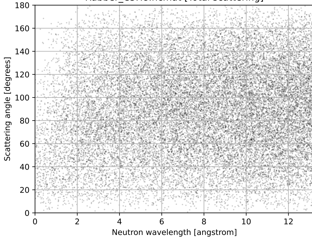
Rubber_C5H8.ncmat [Total scattering]
