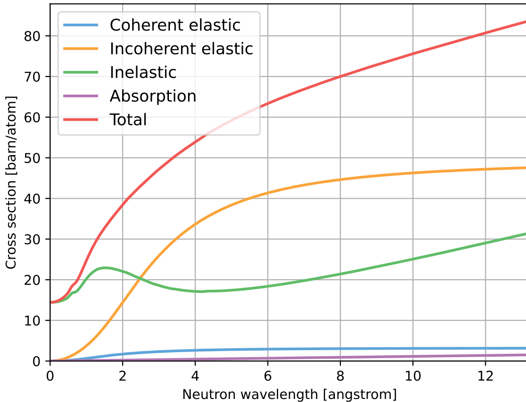
Rubber_C5H8.ncmat
