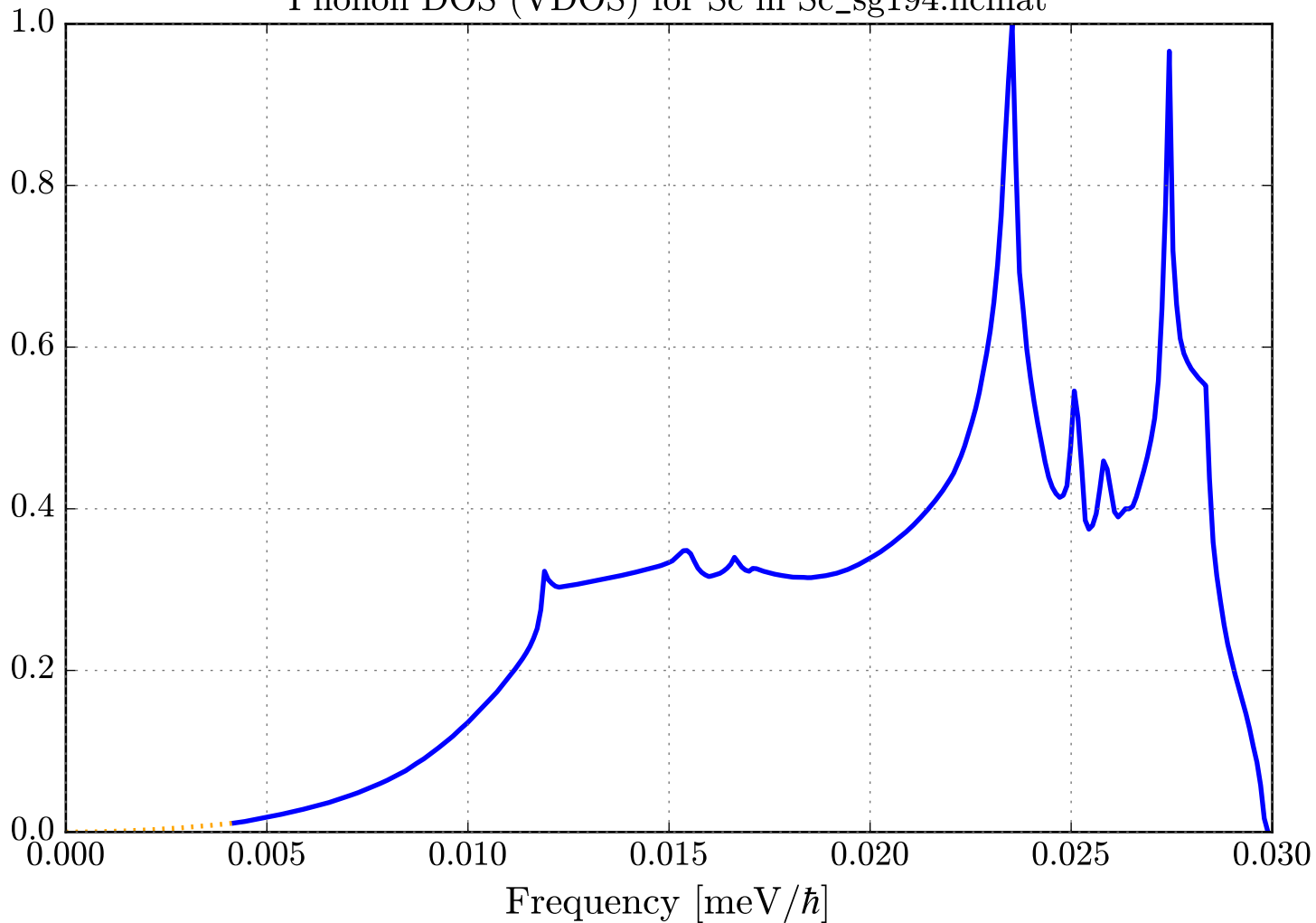
Phonon DOS (VDOS) for Sc in Sc_sg194.ncmat
