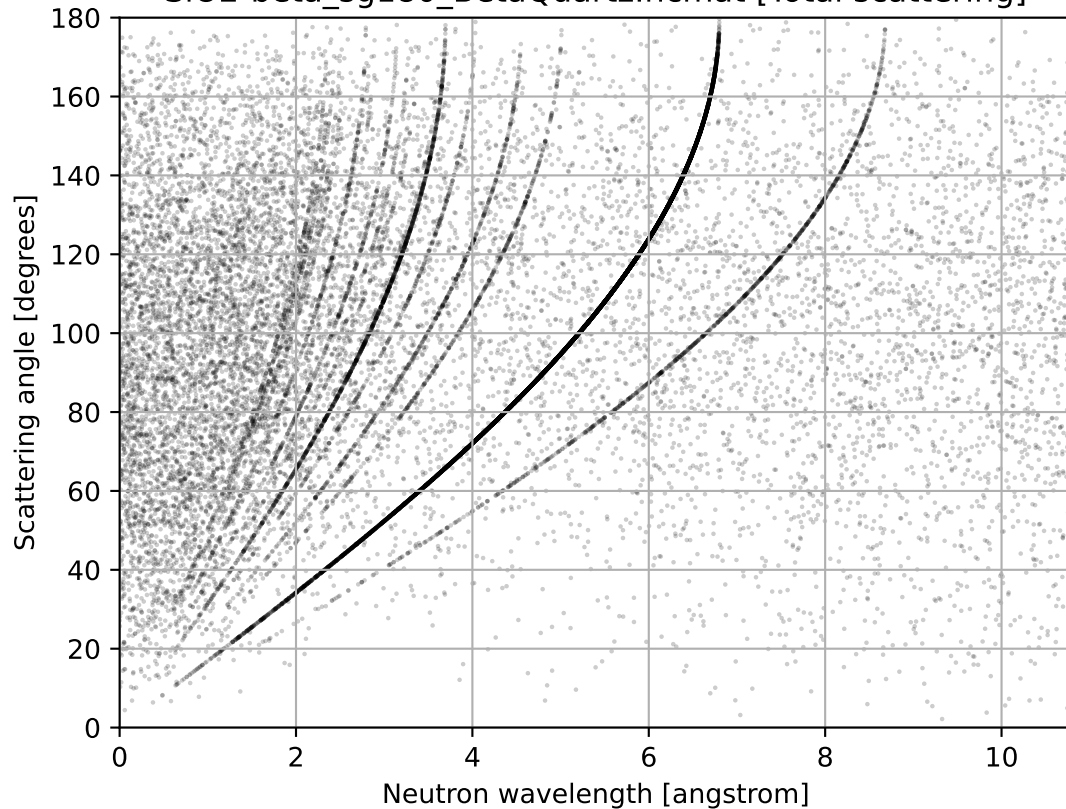
SiO2-beta_sg180_BetaQuartz.ncmat [Total scattering]
