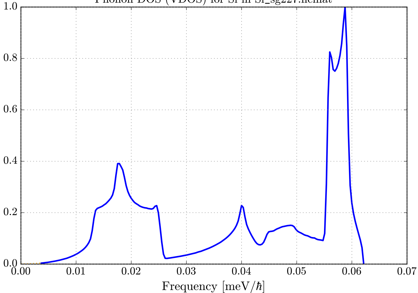
Phonon DOS (VDOS) for Si in Si_sg227.ncmat
