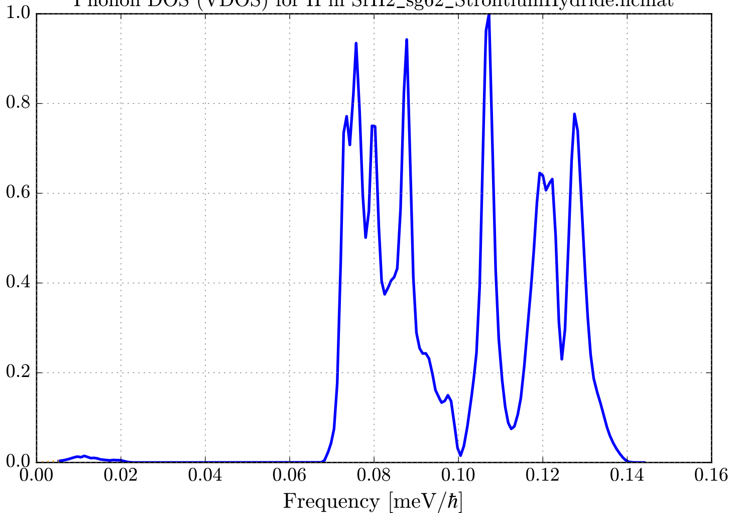
Phonon DOS (VDOS) for H in SrH2_sg62_StrontiumHydride.ncmat
