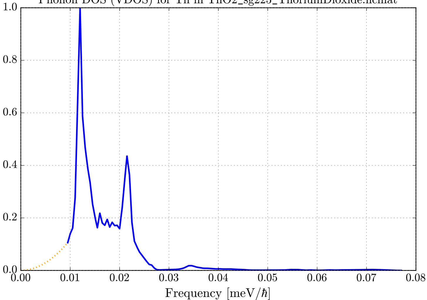
Phonon DOS (VDOS) for Th in ThO2_sg225_ThoriumDioxide.ncmat
