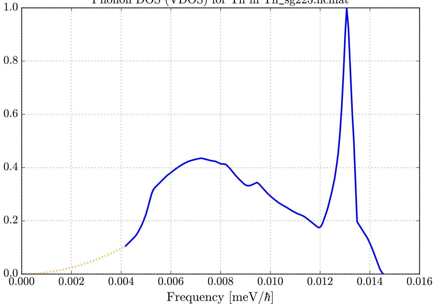
Phonon DOS (VDOS) for Th in Th_sg225.ncmat
