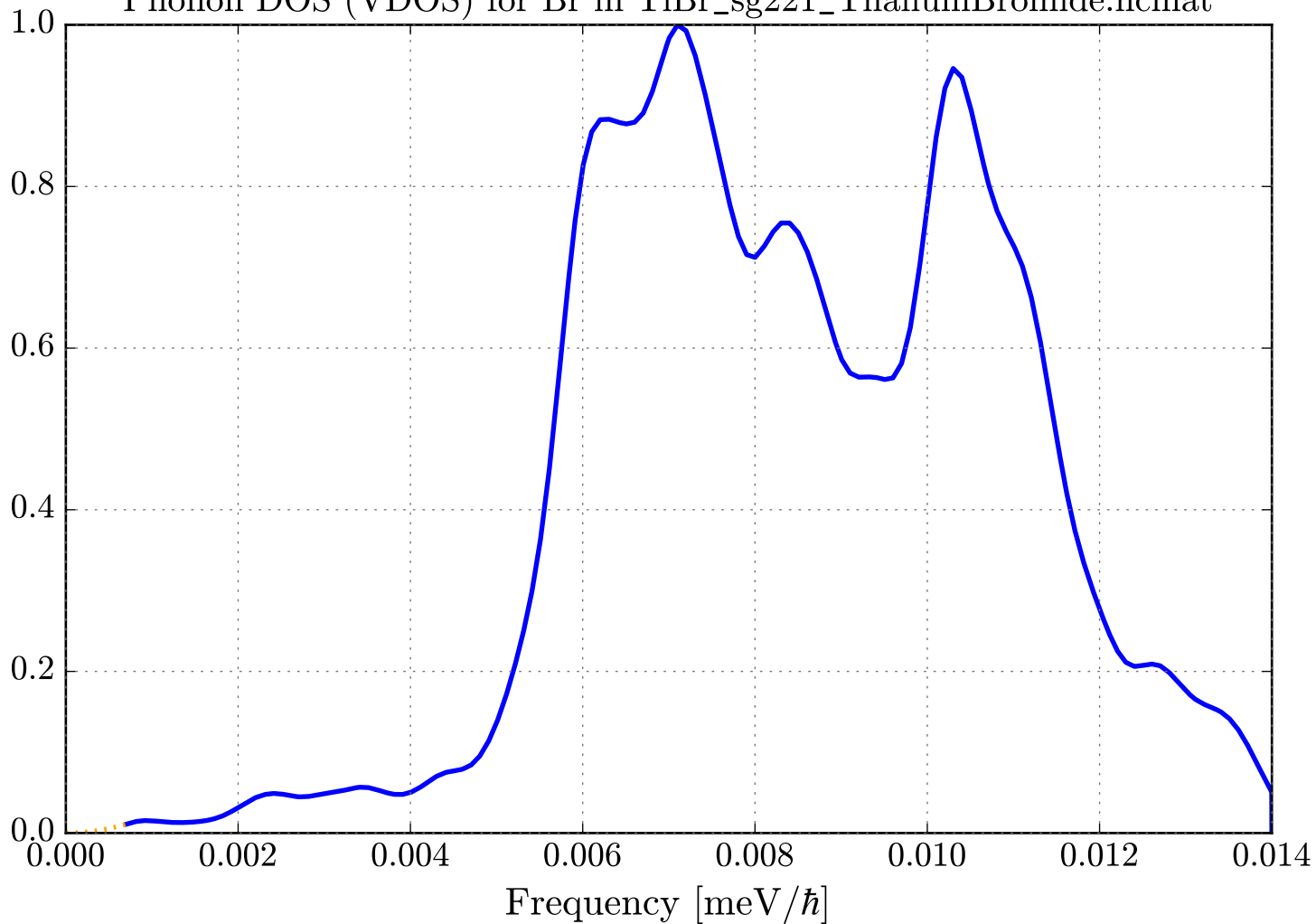
Phonon DOS (VDOS) for Br in TlBr_sg221_ThaliumBromide.ncmat
