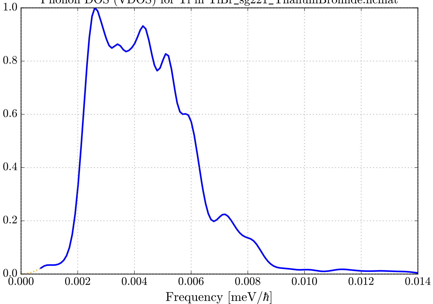
Phonon DOS (VDOS) for Tl in TlBr_sg221_ThaliumBromide.ncmat
