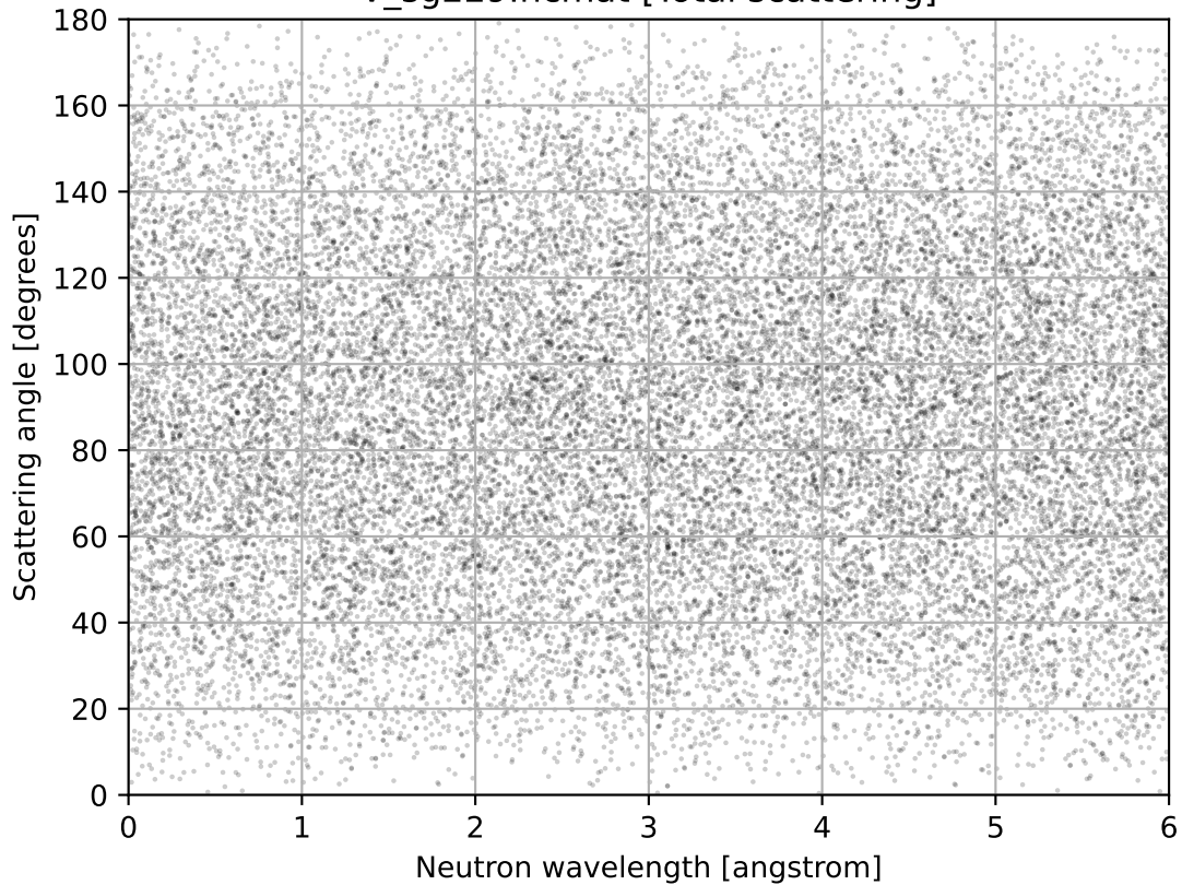
V_sg229.ncmat [Total scattering]
