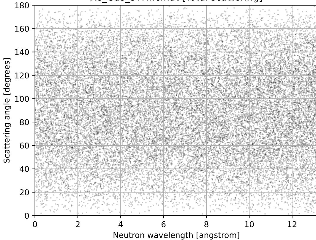
Xe_Gas_STP.ncmat [Total scattering]
