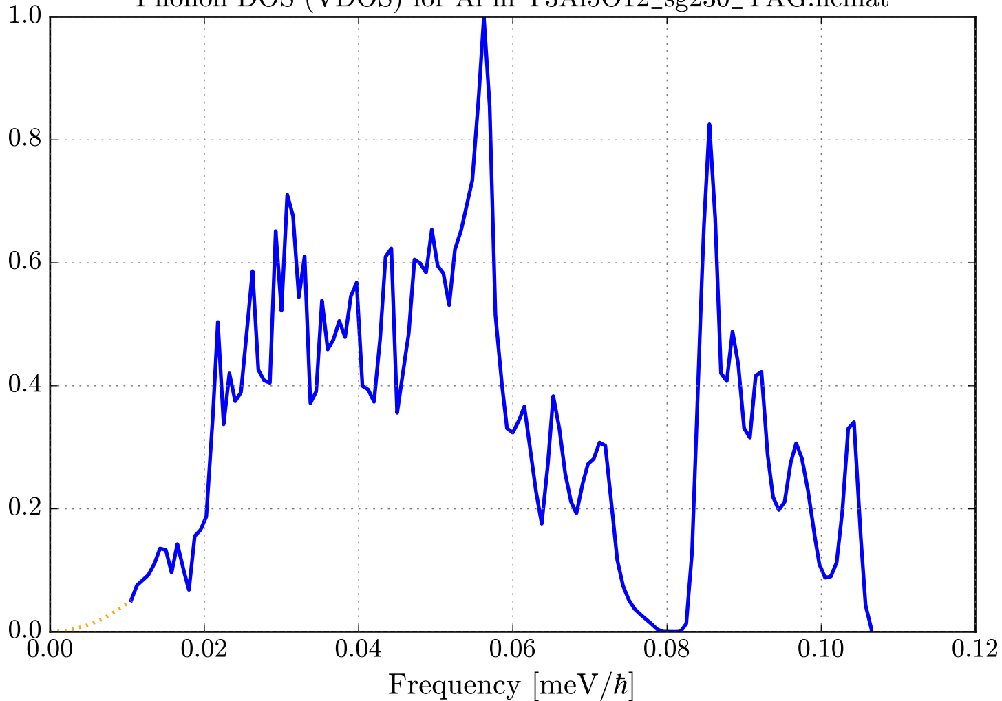
Phonon DOS (VDOS) for Al in Y3Al5O12_sg230_YAG.ncmat
