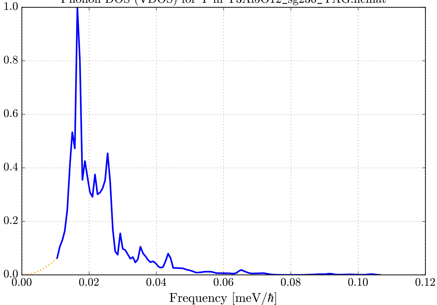
Phonon DOS (VDOS) for Y in Y3Al5O12_sg230_YAG.ncmat
