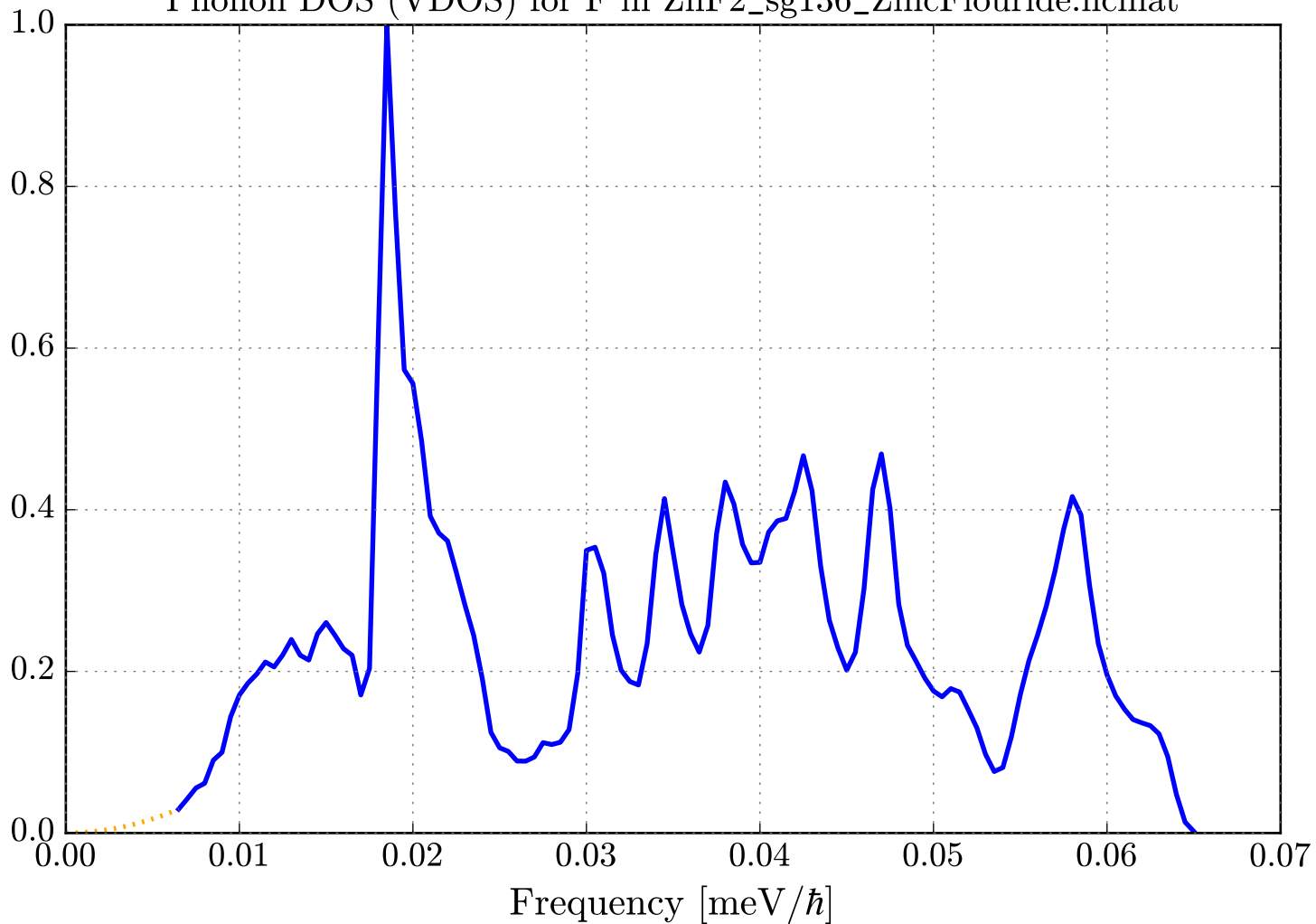
Phonon DOS (VDOS) for F in ZnF2_sg136_ZincFlouride.ncmat
