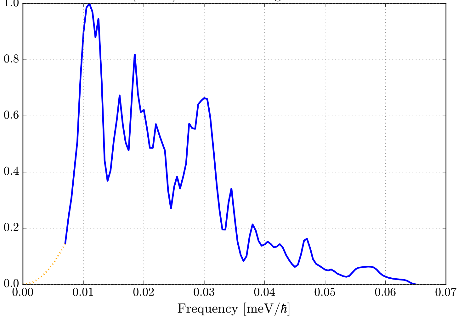
Phonon DOS (VDOS) for Zn in ZnF2_sg136_ZincFlouride.ncmat
