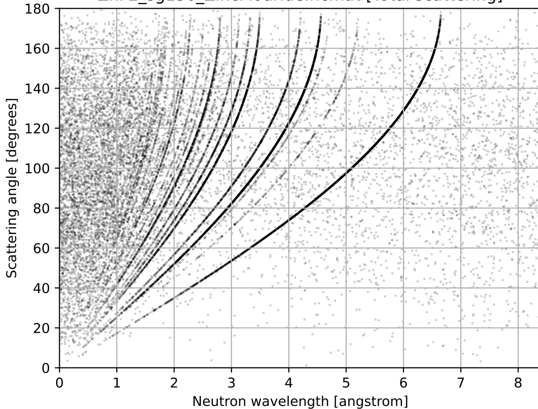
ZnF2_sg136_ZincFlouride.ncmat [Total scattering]
