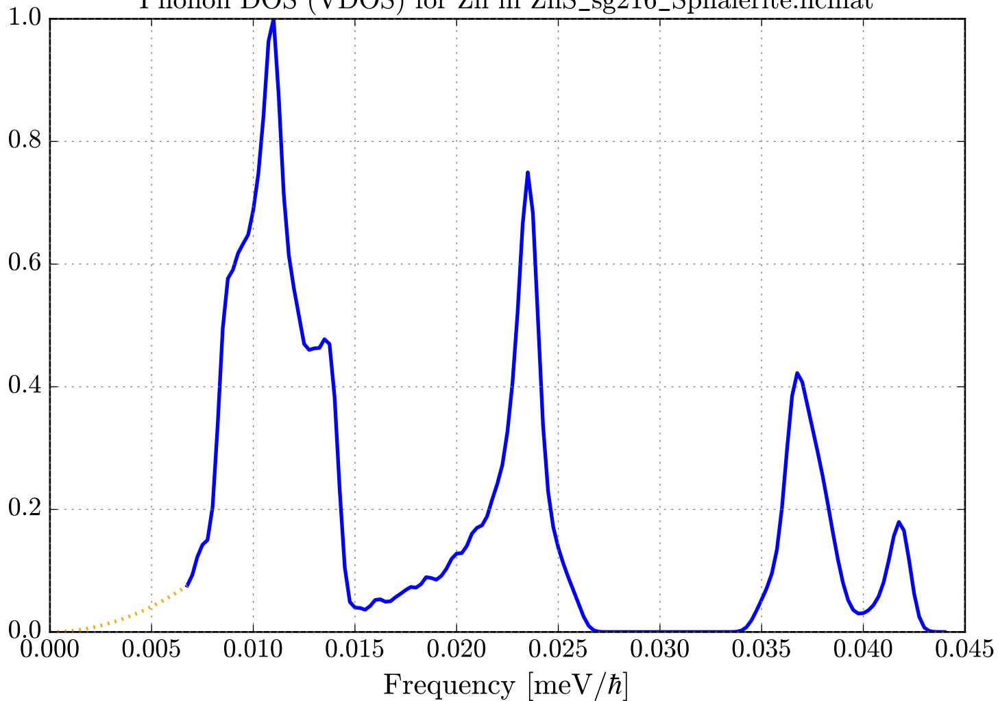
Phonon DOS (VDOS) for Zn in ZnS_sg216_Sphalerite.ncmat
